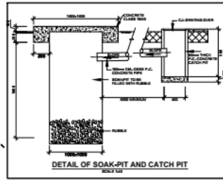
DETAIL OF SOAK-PIT AND CATCH PIT
