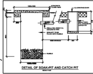
DETAIL OF SOAK-PIT AND CATCH PIT
