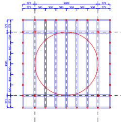
PLATFORM LAYOUT
