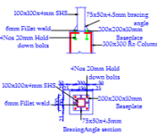
SECT B-B
