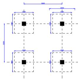
FOUNDATION LAYOUT
