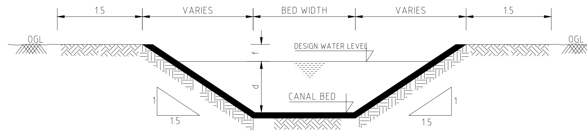
TYPICAL DRAIN CANAL SECTION
