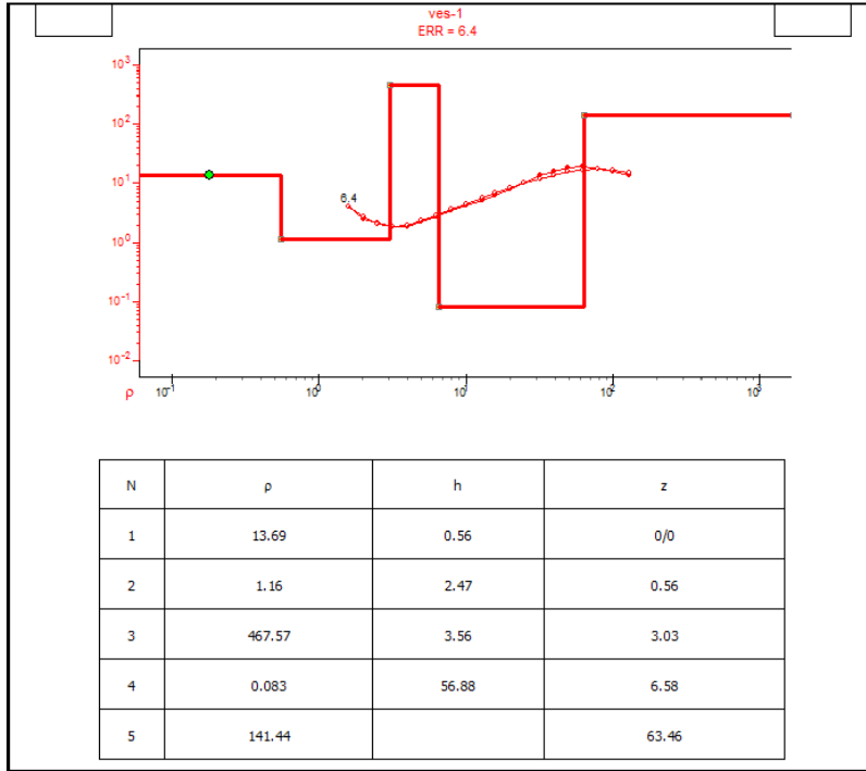
Fig-3: Geo-electric ModelVES-1
